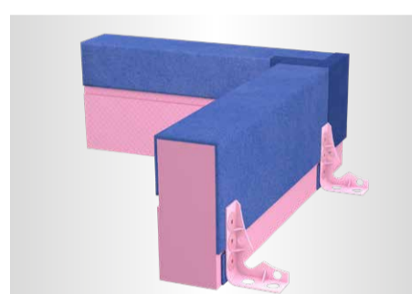
Bodenplattenschalung Thermo System Ecke FBV [ INNENECKE ]
